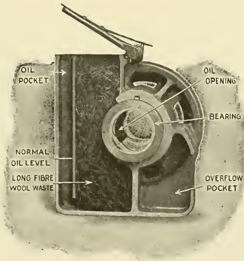
Fig. 41. Cross-Section of Bearing Housing
